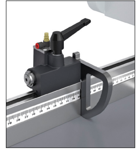
Pneumatic side stop 60 mm (optional).
